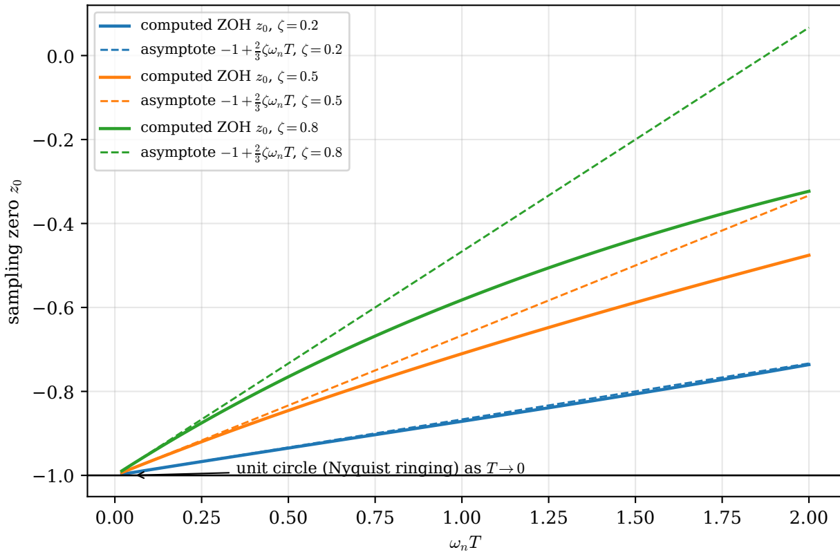
ZOH sampling zero of a relative-degree-2 plant ( z_0 = -b_0/b_1 )
