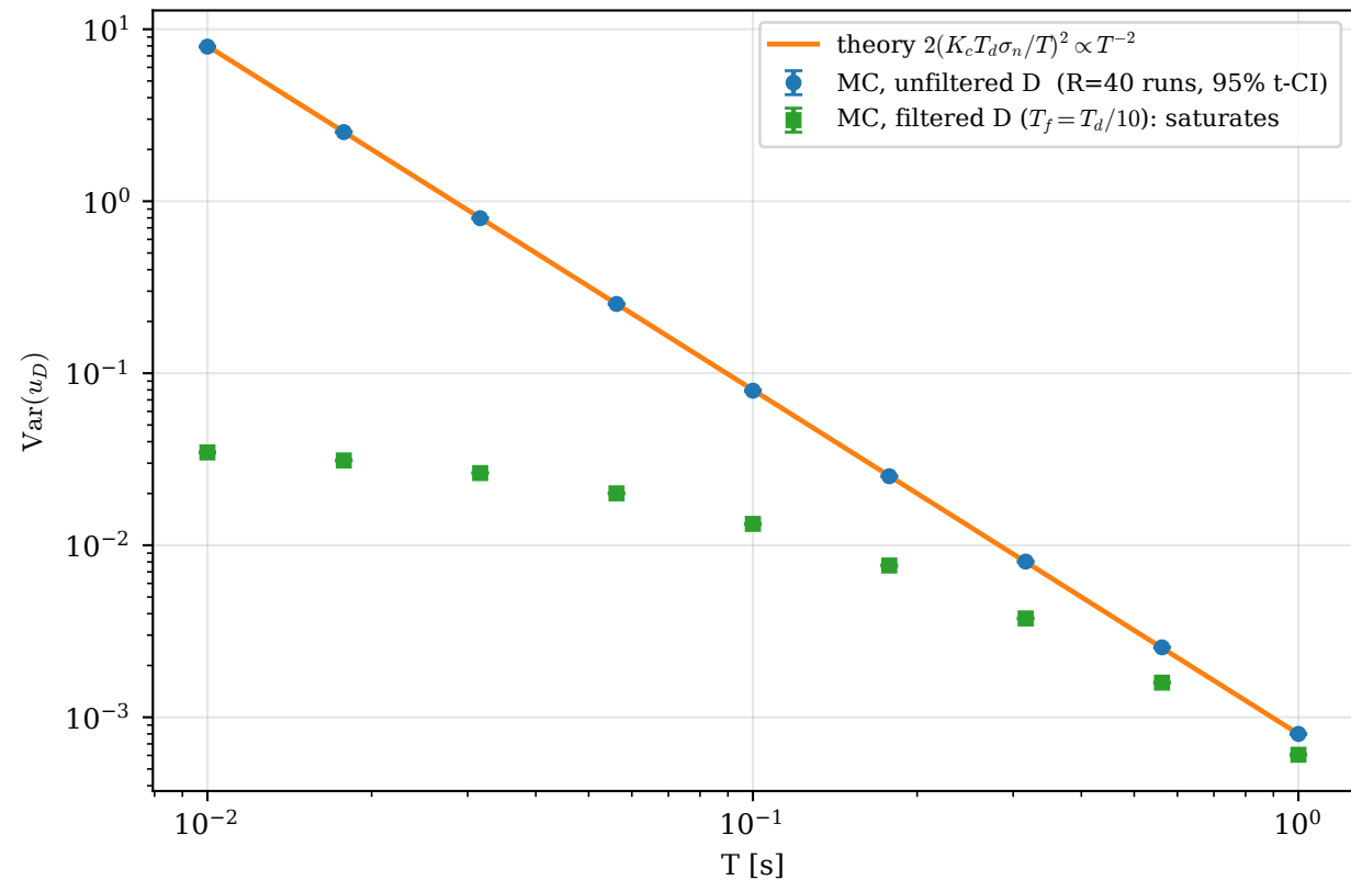
Derivative-term noise amplification vs sampling period
