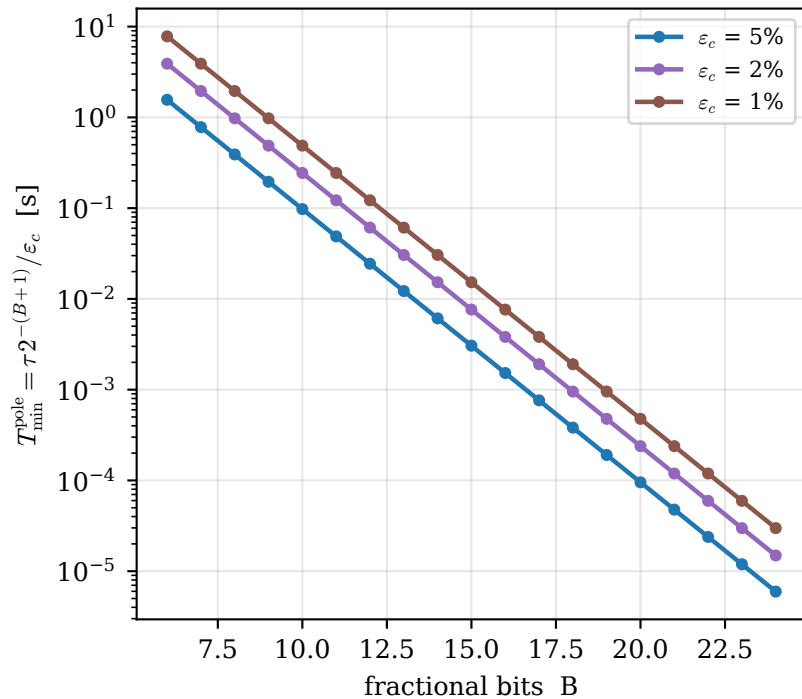
(b) Near-unity pole-resolution bound on T ( \tau = 10 s)
