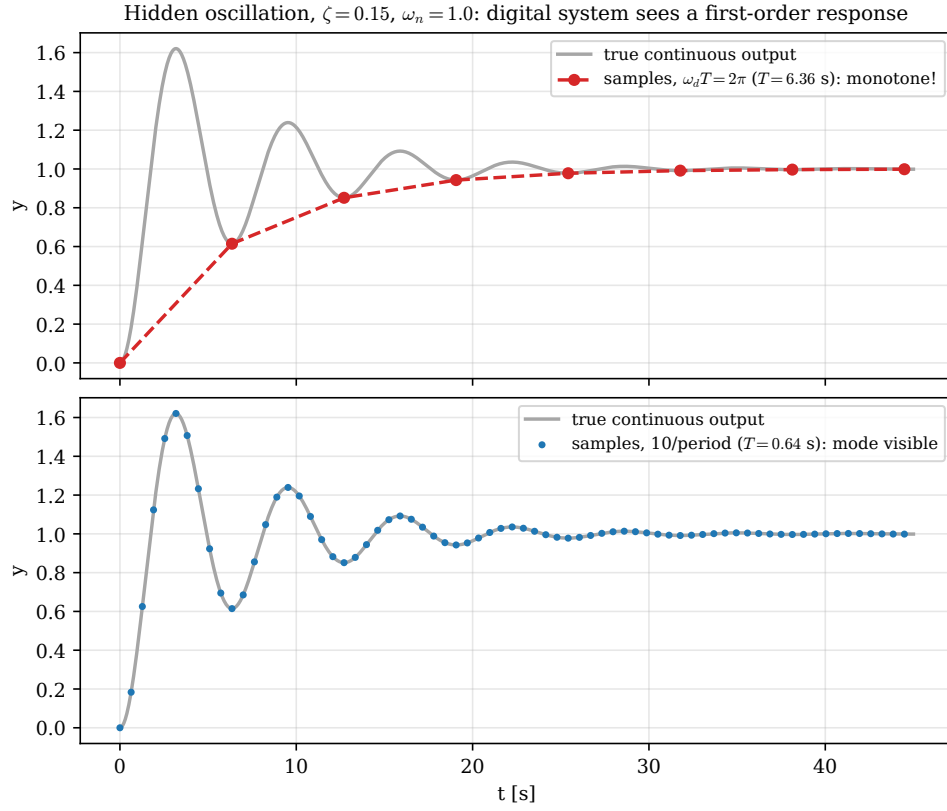
Figure 2: Hidden oscillation for an underdamped SOPTD plant ( \zeta = 0.15 , \omega_n = 1 ). Sampling at \omega_d T = 2\pi (top) yields a monotone sequence that hides a strongly ringing response; ten samples per period (bottom) resolves the mode.
