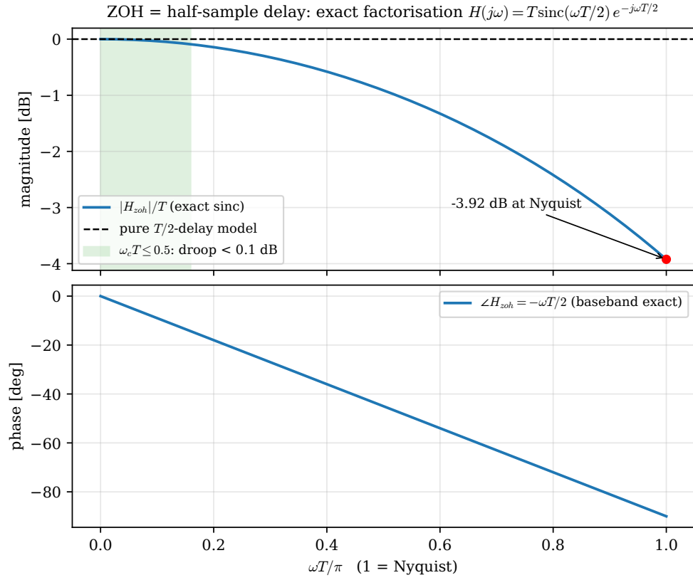
Figure 1: Zero-order hold as an effective half-sample delay (Lemma 1). The baseband phase is exactly -\omega T/2 ; the magnitude droop stays below 0.1 dB for \omega T \leq 0.5 and reaches -3.9 dB only at the Nyquist frequency.
