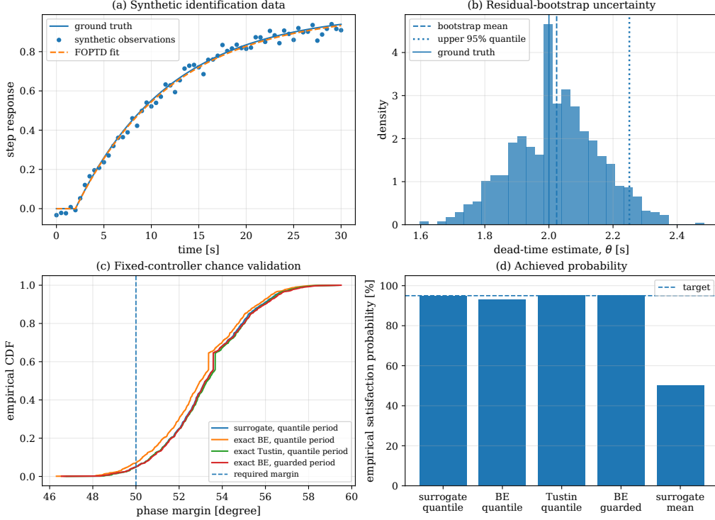
Figure 10: Synthetic uncertainty study. (a) Noisy step data and fitted FOPTD model. (b) Residual-bootstrap dead-time distribution. (c) Empirical phase-margin distributions for the quantile period and a backward-Euler guard period. (d) Achieved probability compared with the 95% target.
