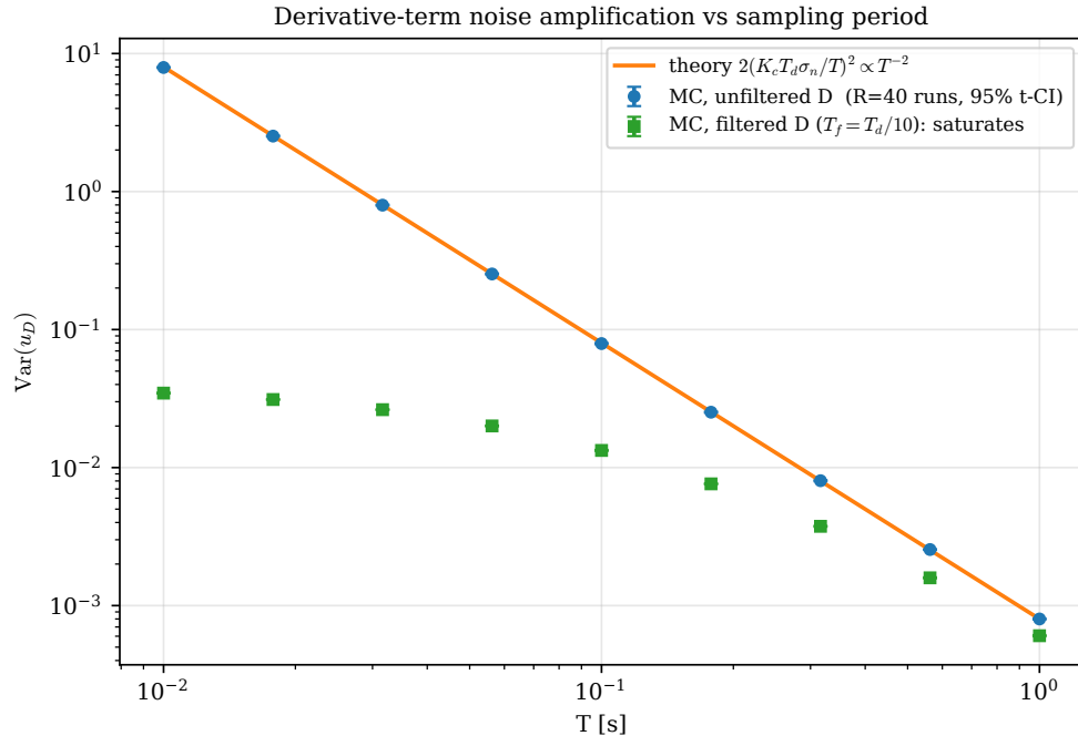
Figure 9: Derivative-term noise amplification. The unfiltered variance follows T^{-2} ; a first-order filtered derivative limits the high-frequency gain.
