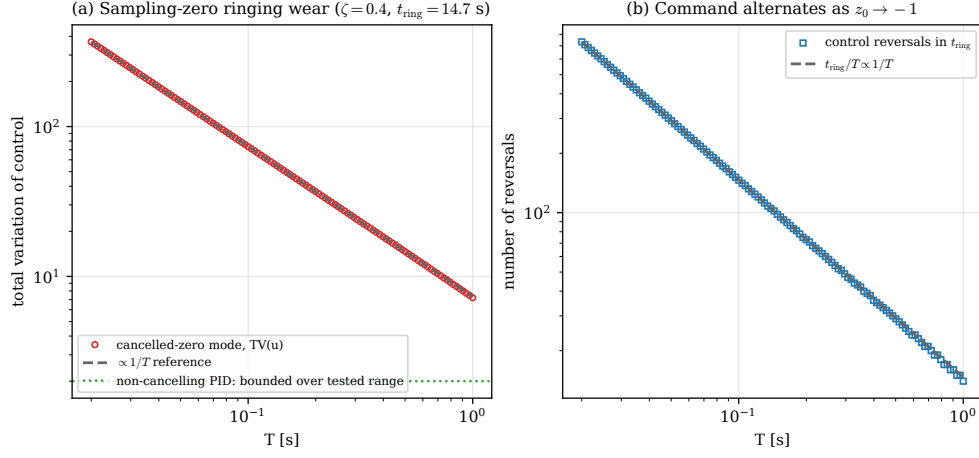
Figure 4: Command variation for a cancelled sampling-zero mode ( \zeta = 0.4 ). Total variation (a) and the number of control reversals (b) both scale as 1/T ; a non-cancelling PID keeps the variation bounded and approximately T -independent over the tested range.
