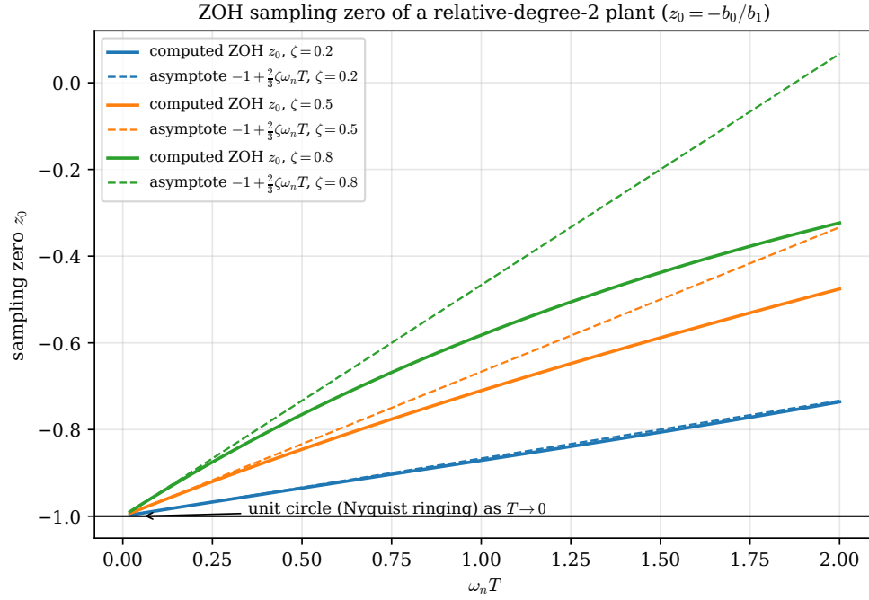
Figure 3: Sampling zero of the relative-degree-two plant against the first-order expansion Eq. (31). The zero converges to z = -1 as T \rightarrow 0 for every damping ratio.
