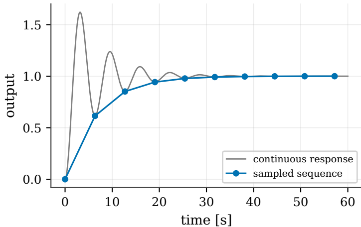
(a) \omega_d T = 2\pi : ringing hidden
