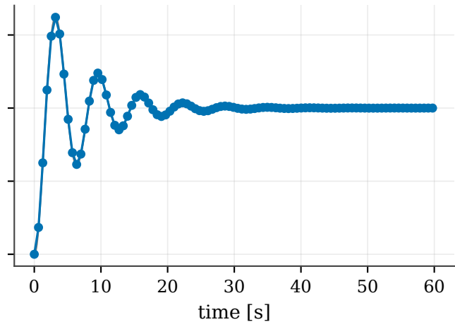
(b) ten samples per damped period
