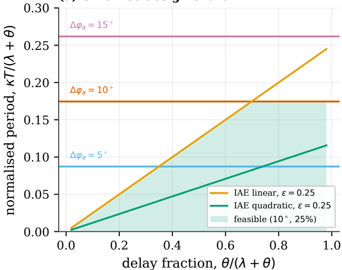
(a) Unit-free design chart
