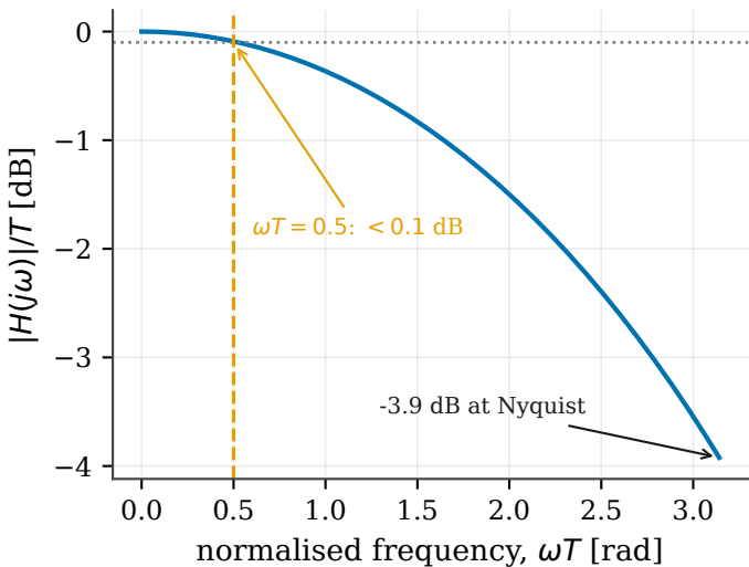
(a) Hold magnitude droop
