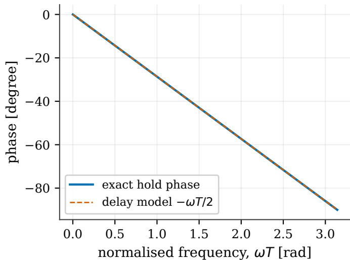
(b) Phase is exactly a half sample
