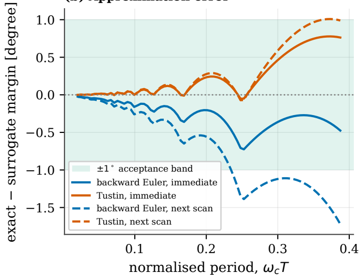
(b) Approximation error
