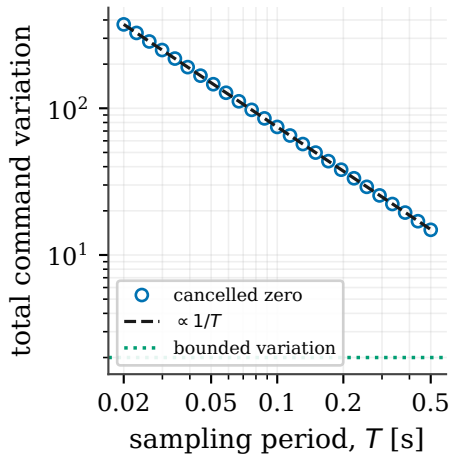
(b) Command travel, \zeta = 0.4
