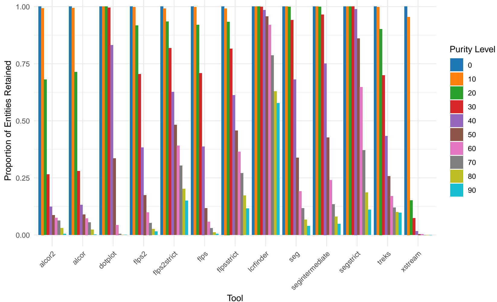
Proportion of Entities Retained per Tool at Different Purities
