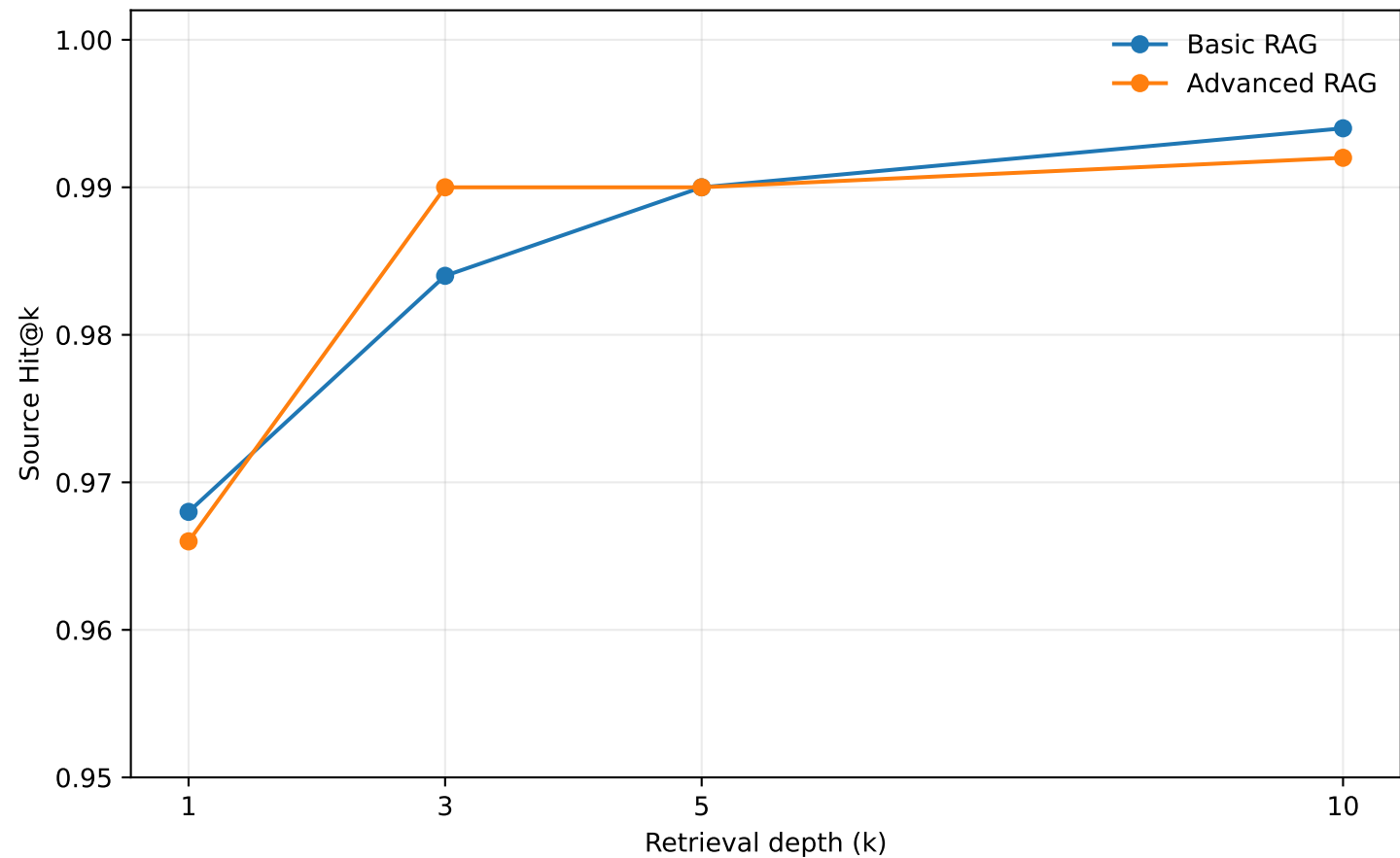
Correct-source retrieval on the final test set
