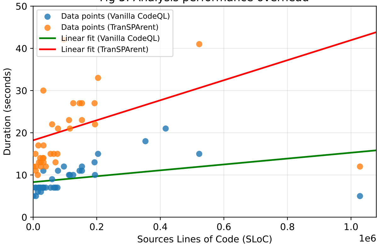
Fig 5: Analysis performance overhead
