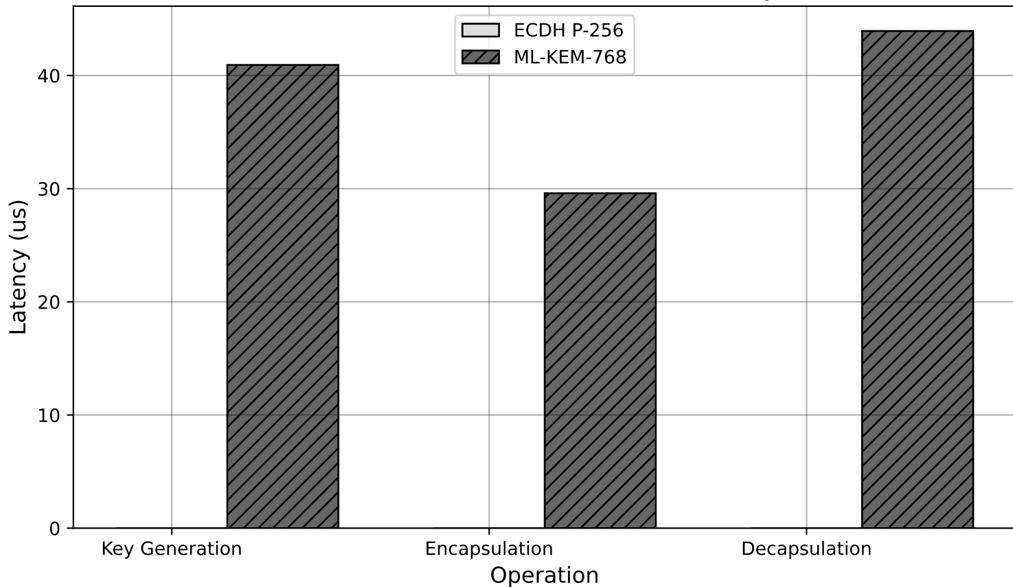
ECDH P-256 vs ML-KEM-768 (Latency)
