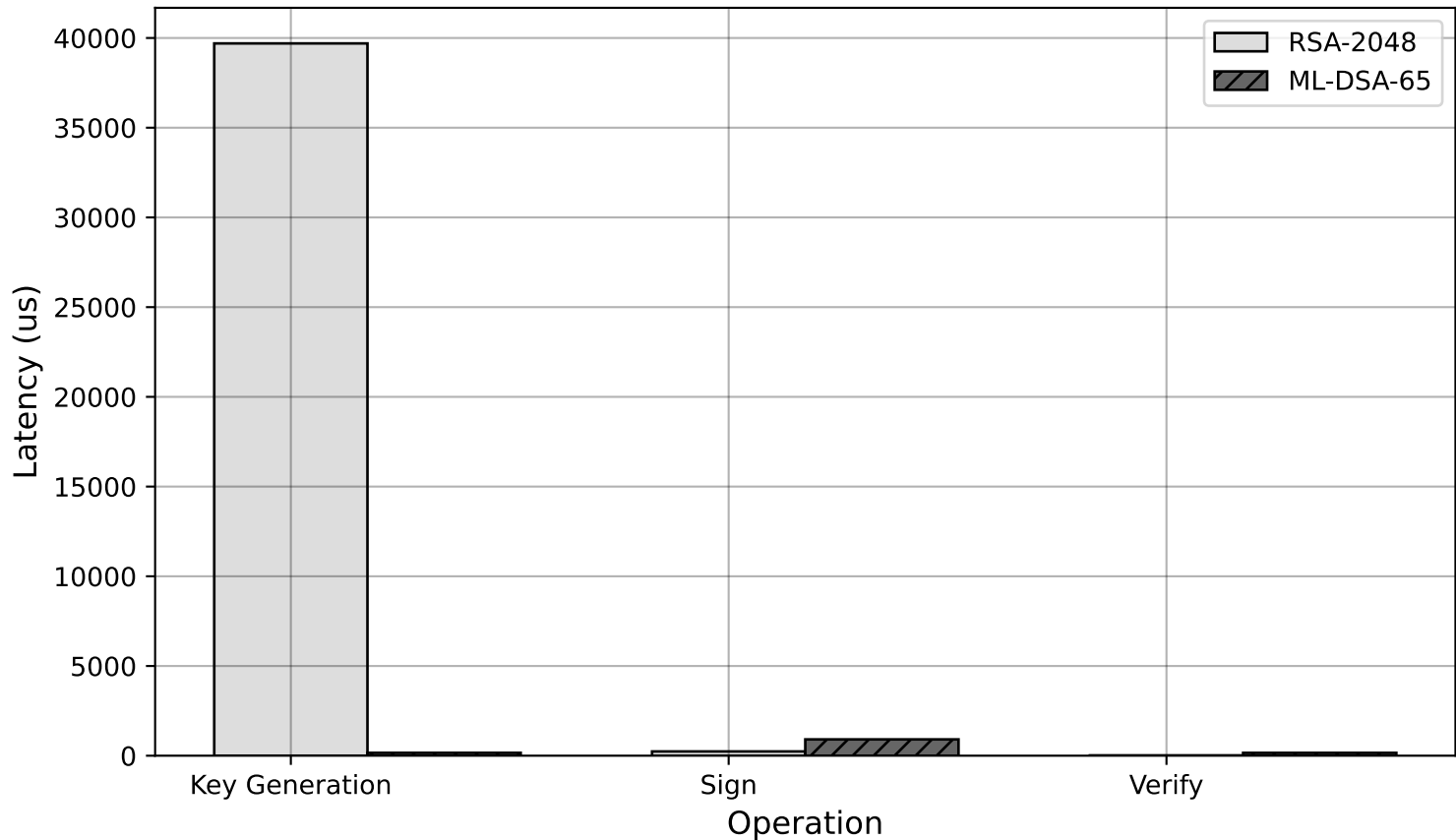
RSA-2048 vs ML-DSA-65 (Latency)
