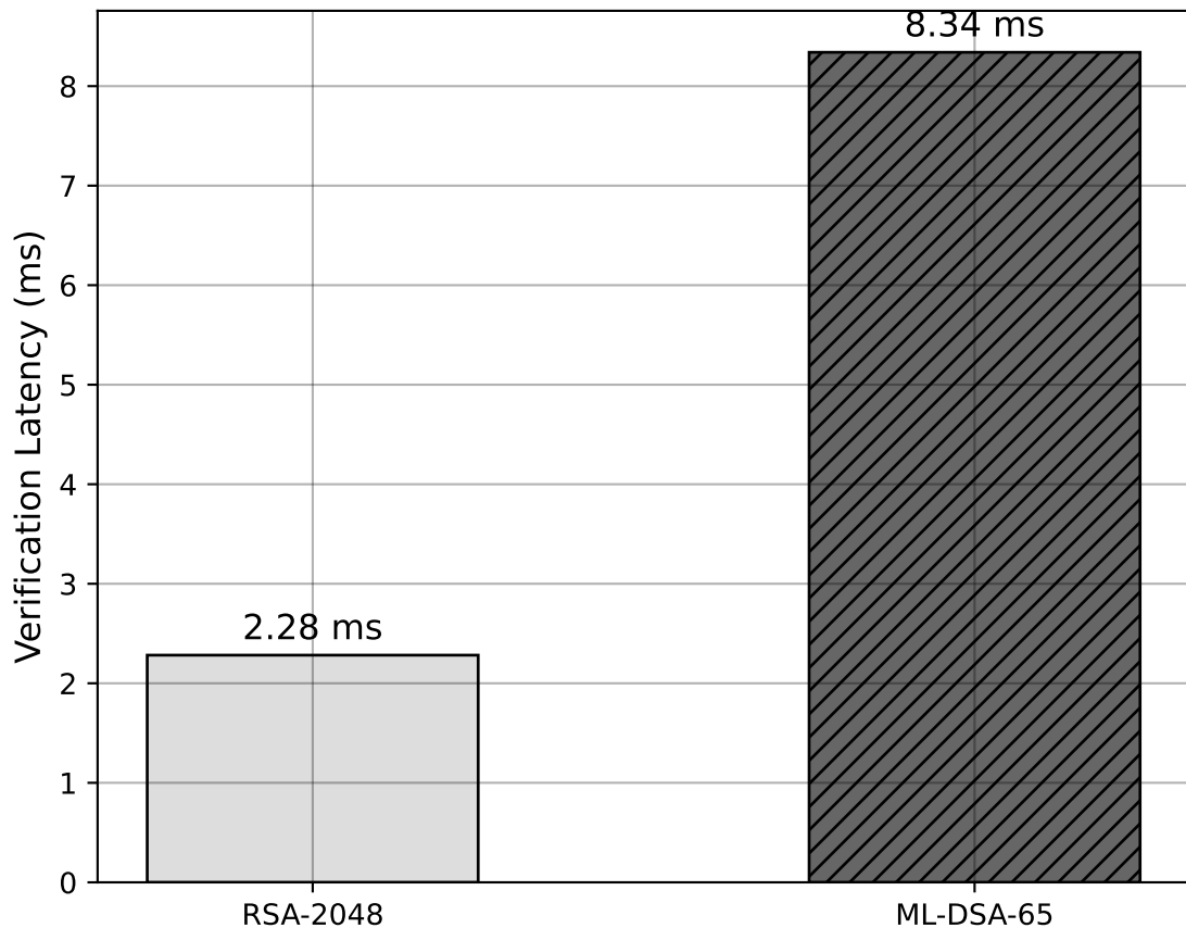
Secure Boot Simulation (4MB Kernel)
