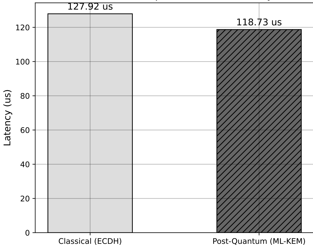
Secure IPC Roundtrip Simulation (4KB Payload)
