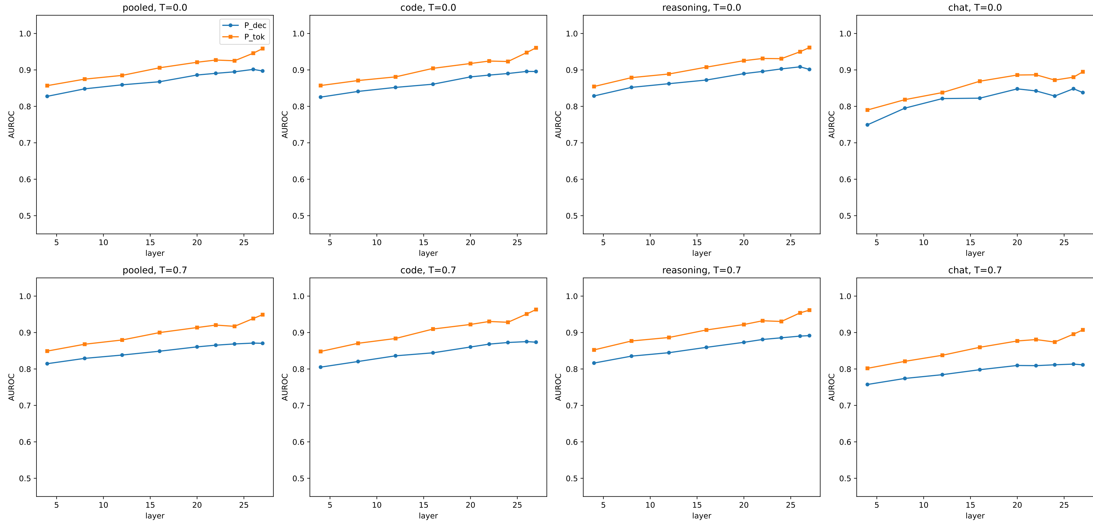
E2: P_dec vs P_tok, AUROC by layer
