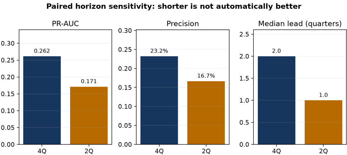
Figure 1. The two-quarter label reduces queue size but loses ranking quality, precision, and warning time.
