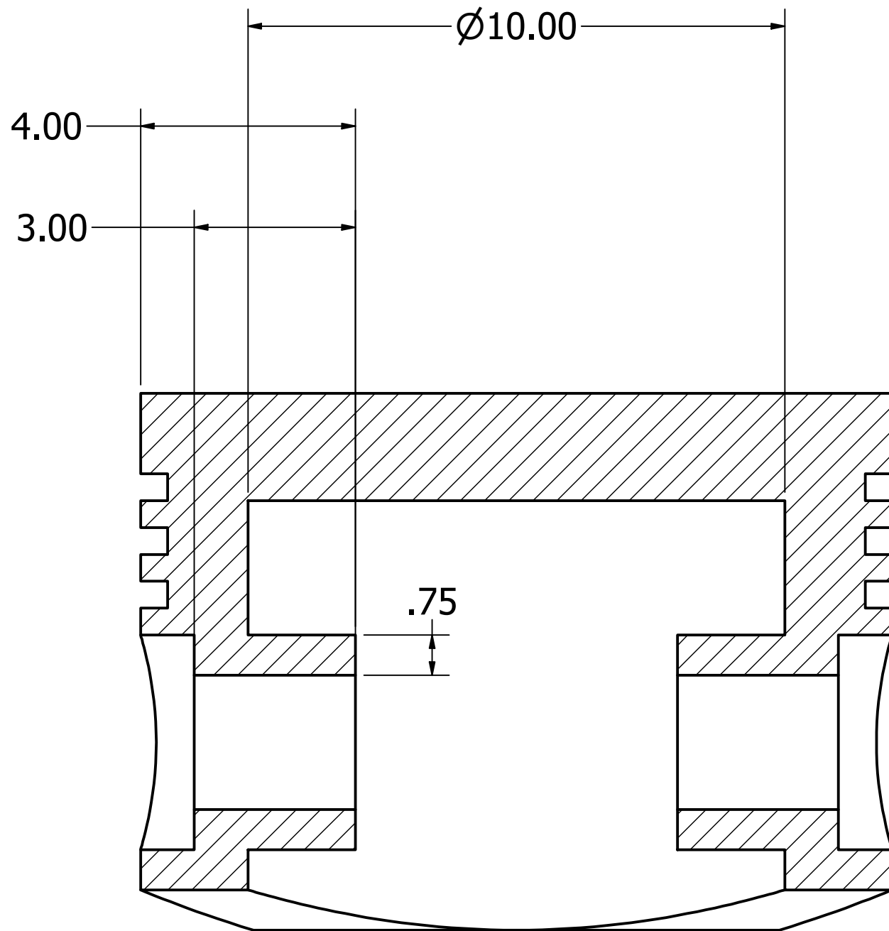
SECTION F-F SCALE 10
