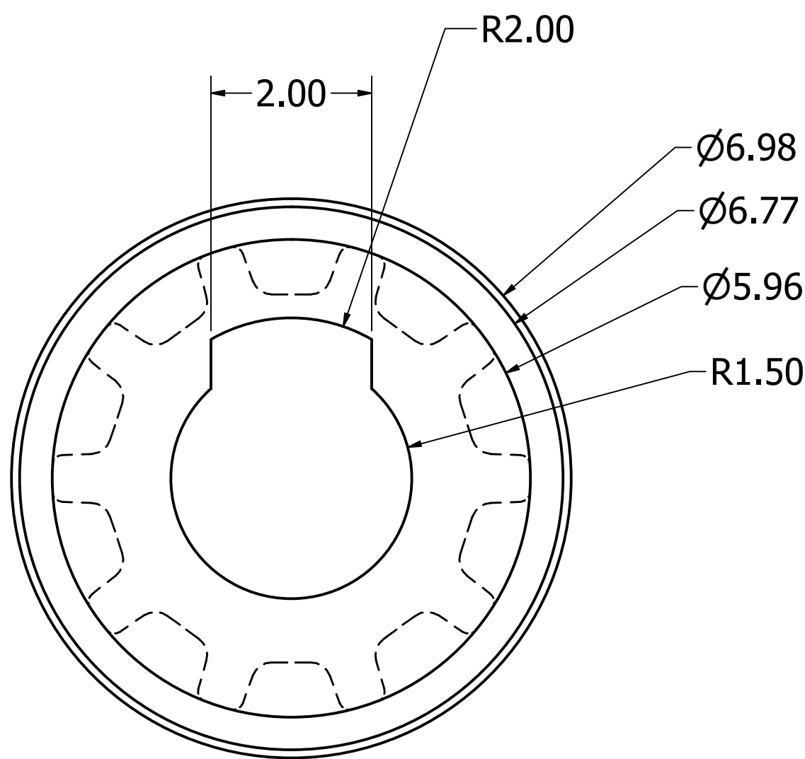
SECTION H-H SCALE 15: 1
