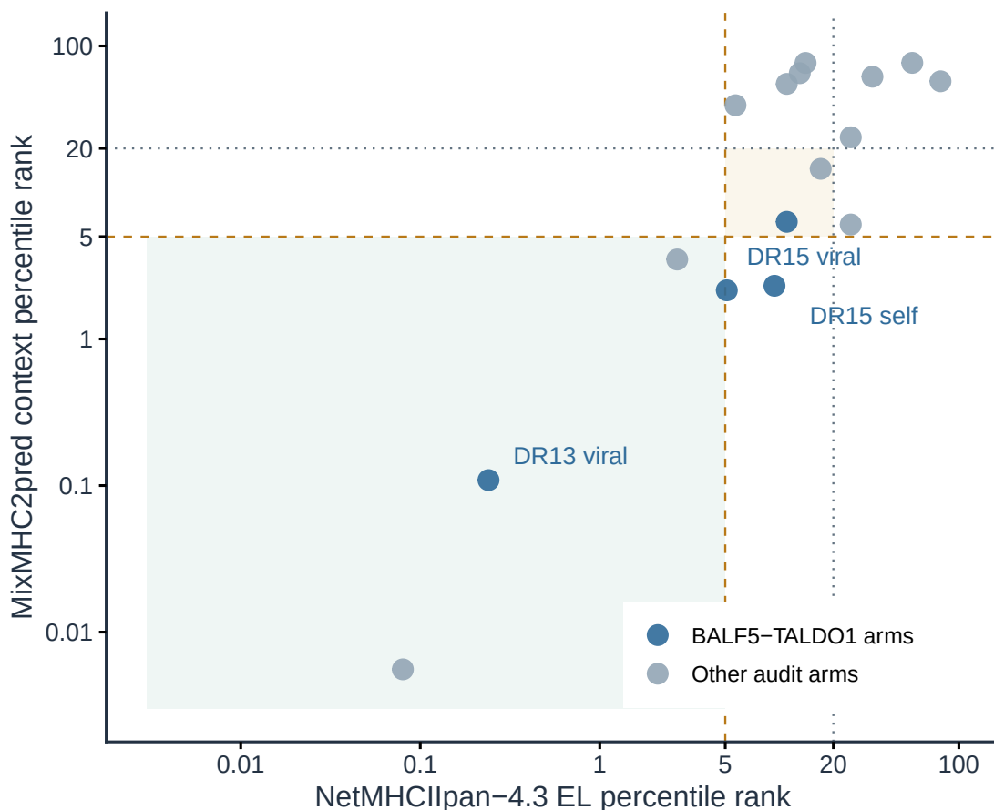
Figure 5: Concordance of peptide–HLA class II binding-predictions in the initial eight-pair audit. Each point represents one peptide arm. NetMHCIIpan-4.3 EL and MixMHC2pred context percentile ranks are plotted on logarithmic axes; lower values indicate stronger predicted binding. Gold dashed lines mark the \leq 5\% full-consensus threshold, gray dotted lines mark the \leq 20\% lesser-support threshold, and the shaded region identifies arms below 5% in both predictors. Blue points are BALF5–TALDO1 arms; gray points are other audited arms.
