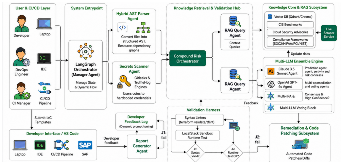
Fig. 1. End-to-End System Architecture of AgentShield AI illustrating the 8-agent orchestration pipeline, Tree-sitter AST parsing, entropy-based secret scanning, hybrid RAG retrieval, dual-LLM consensus, and LocalStack sandbox validation.
