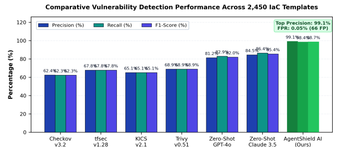
Fig. 2. Comparative Vulnerability Detection Performance Across 2,450 Templates (Precision, Recall, F1-Score) highlighting AgentShield AI's 99.1% precision and 0.05% FPR.
