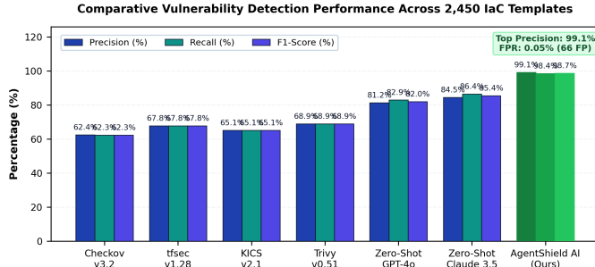
Fig. 2. Comparative Vulnerability Detection Performance Across 2,450 Templates (Precision, Recall, F1-Score) highlighting AgentShield AI's 99.1% precision and 0.05% FPR.
