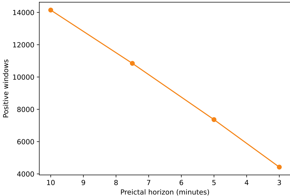
Positive class size vs horizon
