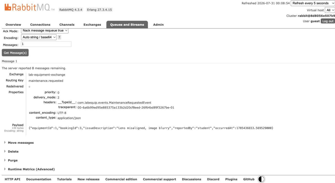
Figure 10: Actual MaintenanceRequested message payload, inspected via RabbitMQ
