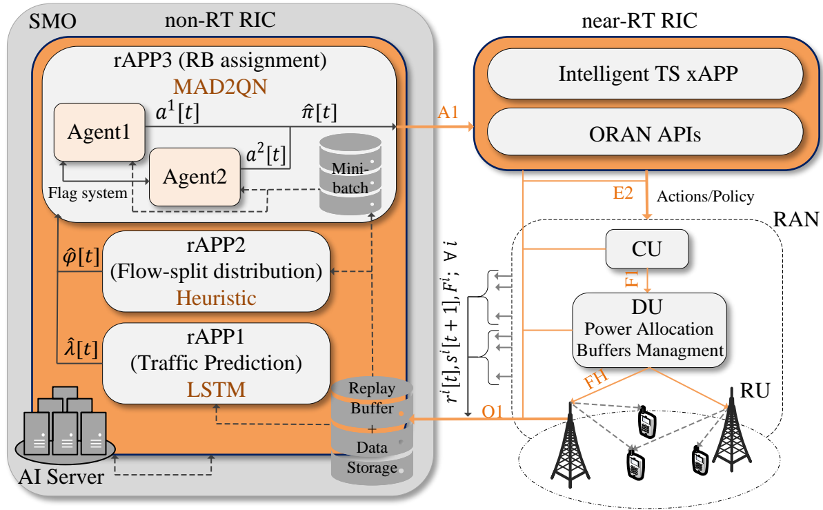
(b) The streamlined workflow for deploying ML applications in the Open RAN architecture.
