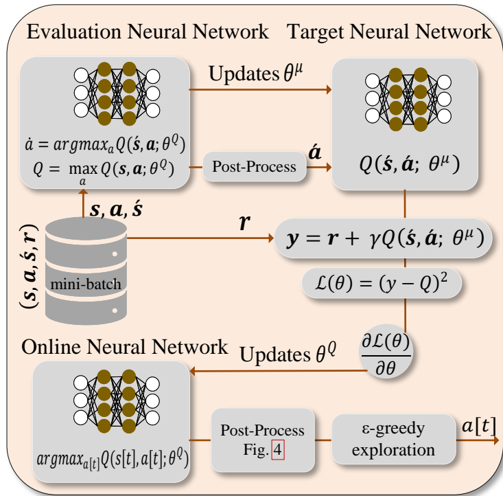
(a) Structure of Double DQN (D2QN) agent
