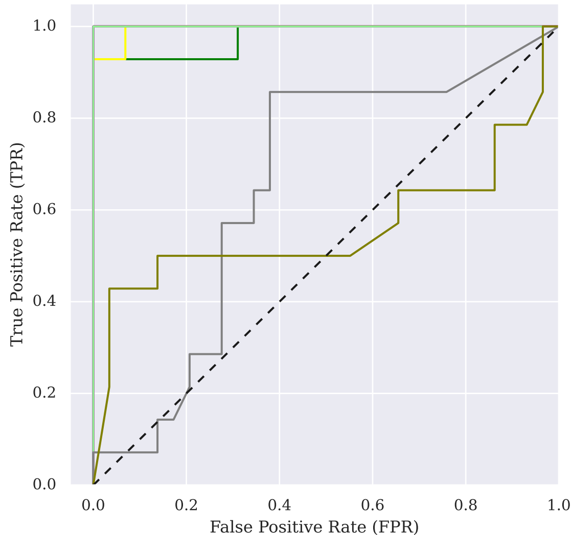
ROC Curve
