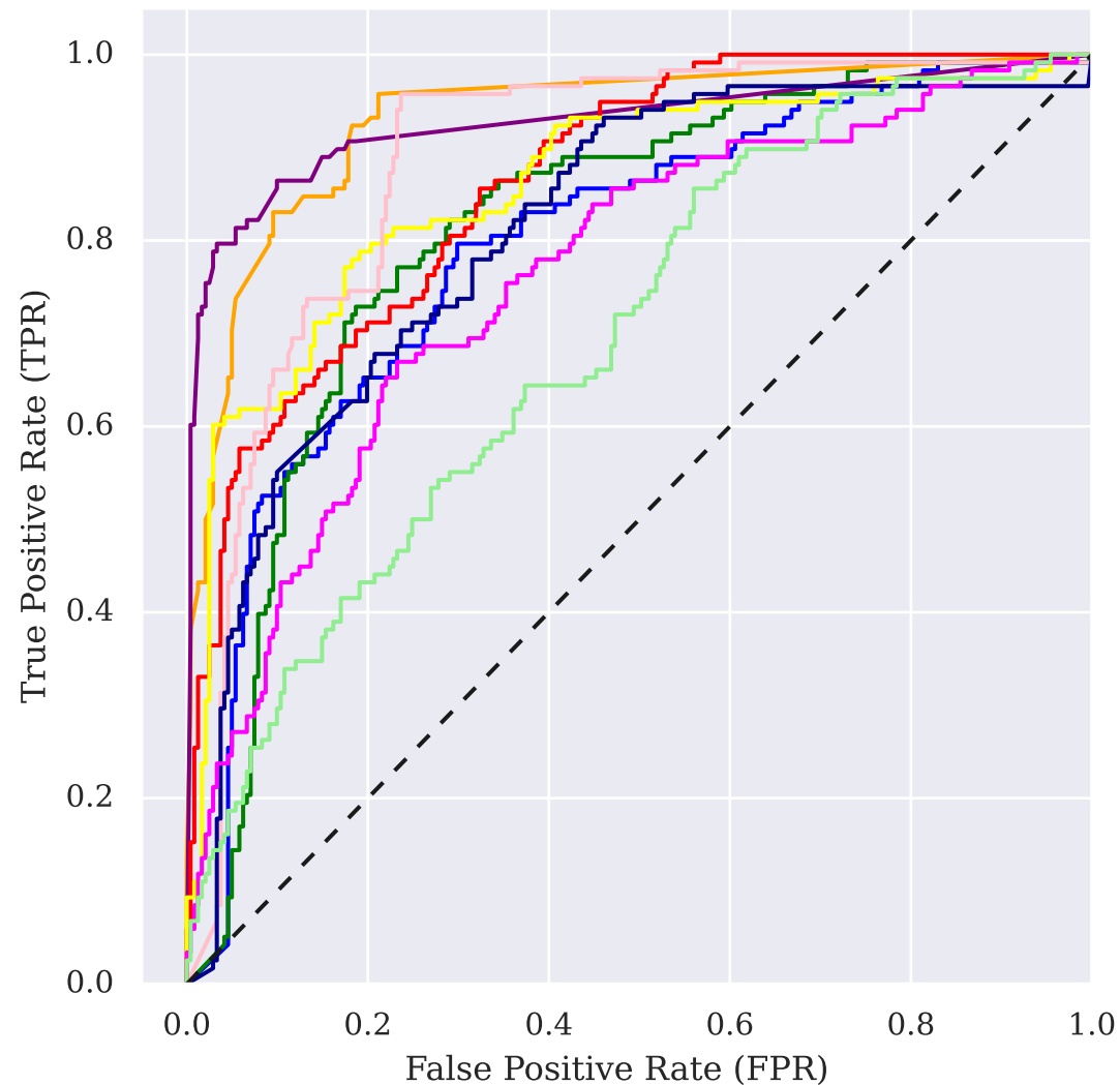
ROC Curve
