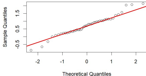
QQ Plot X 3
