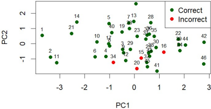
Clustering vs true class
