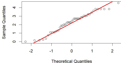
QQ Plot X 2
