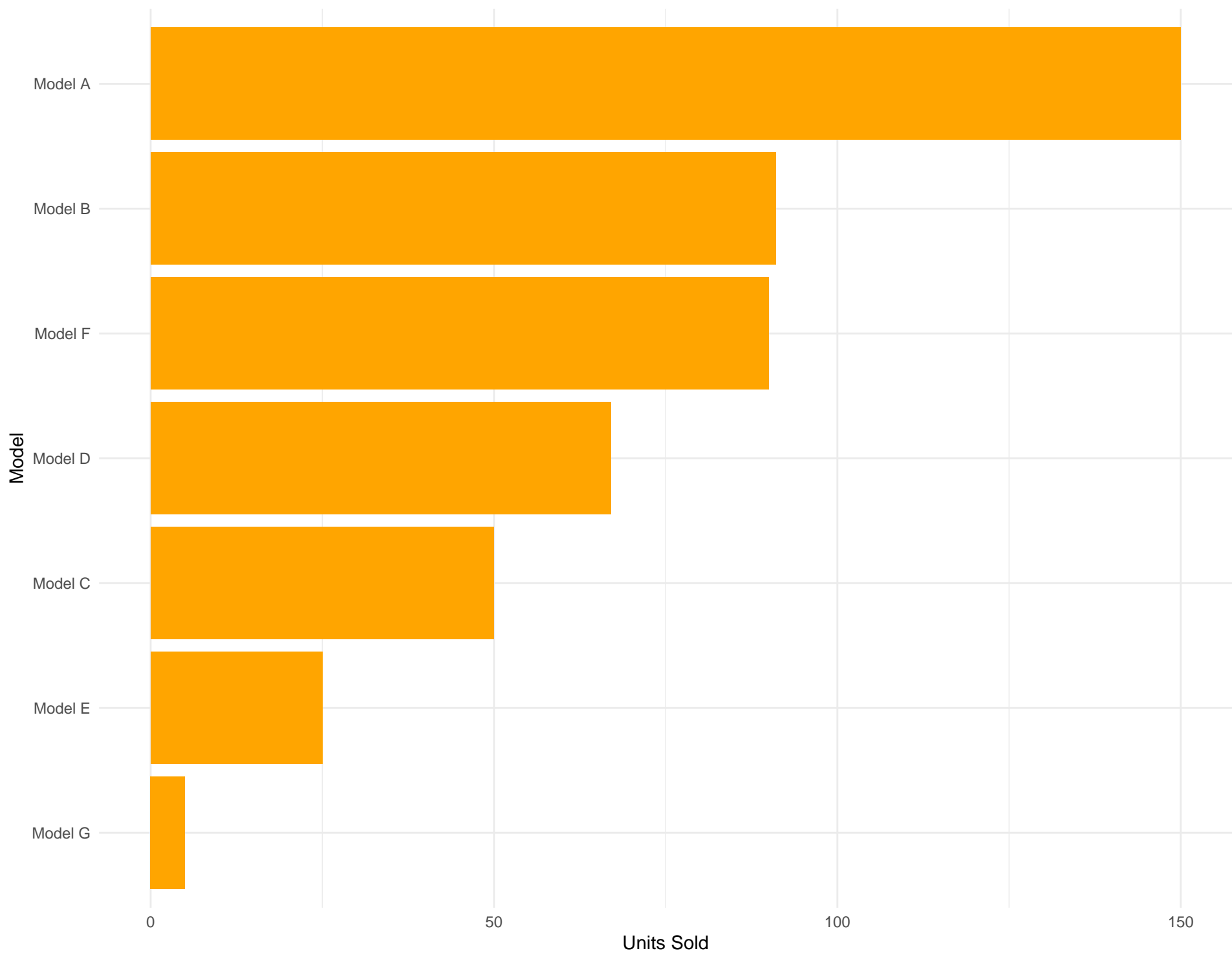
Bar Plot: Units Sold by Model
