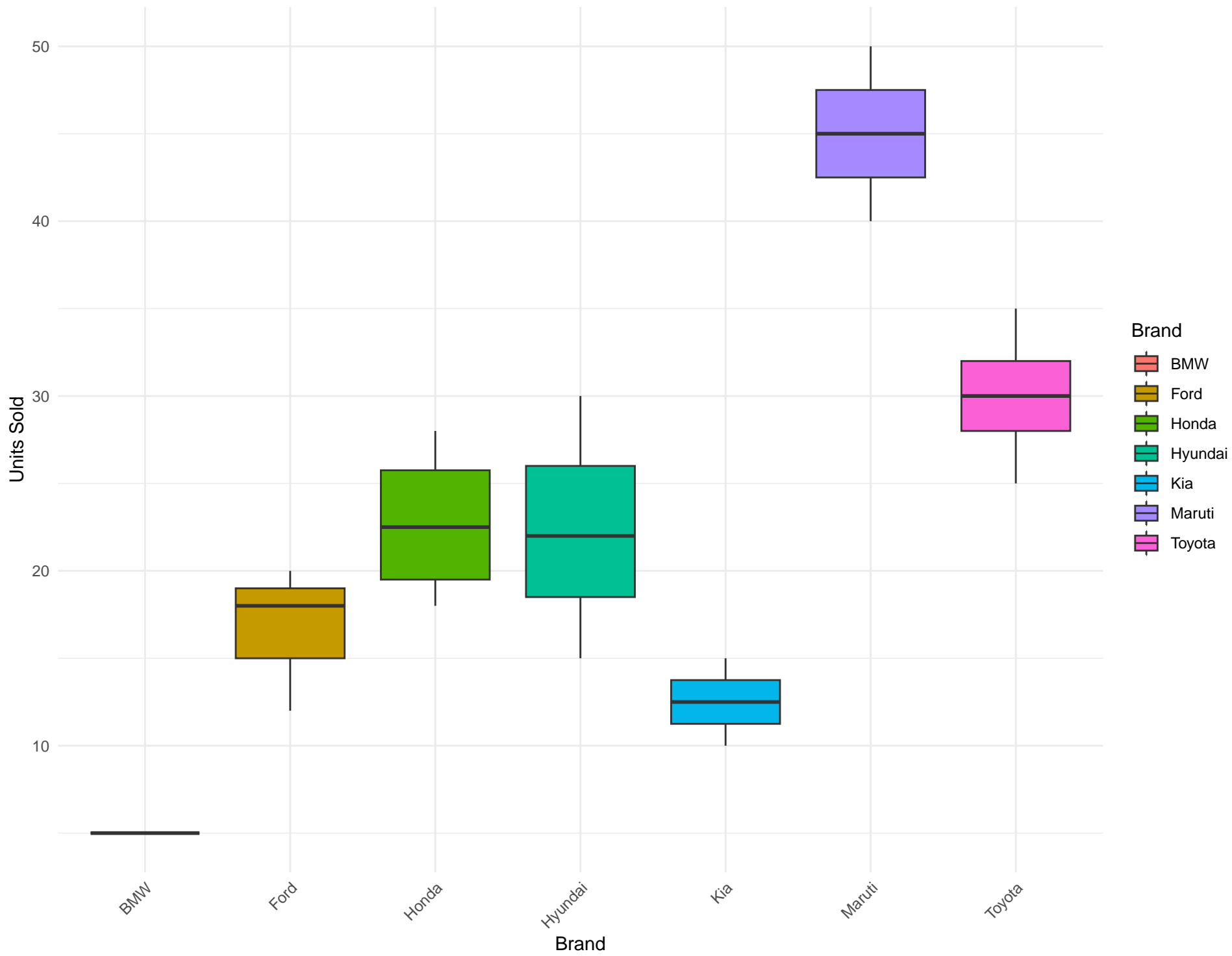
Box Plot: Units Sold by Brand
