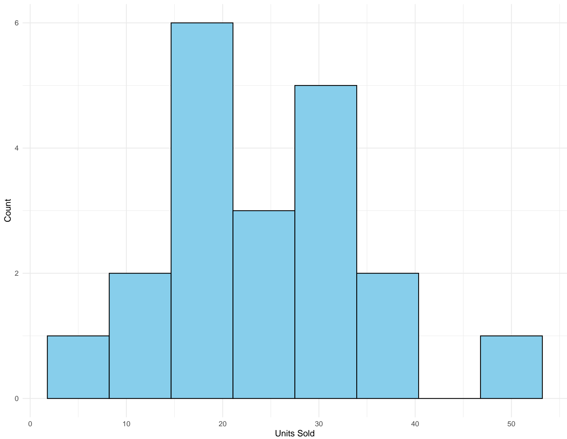
Histogram of Units Sold
