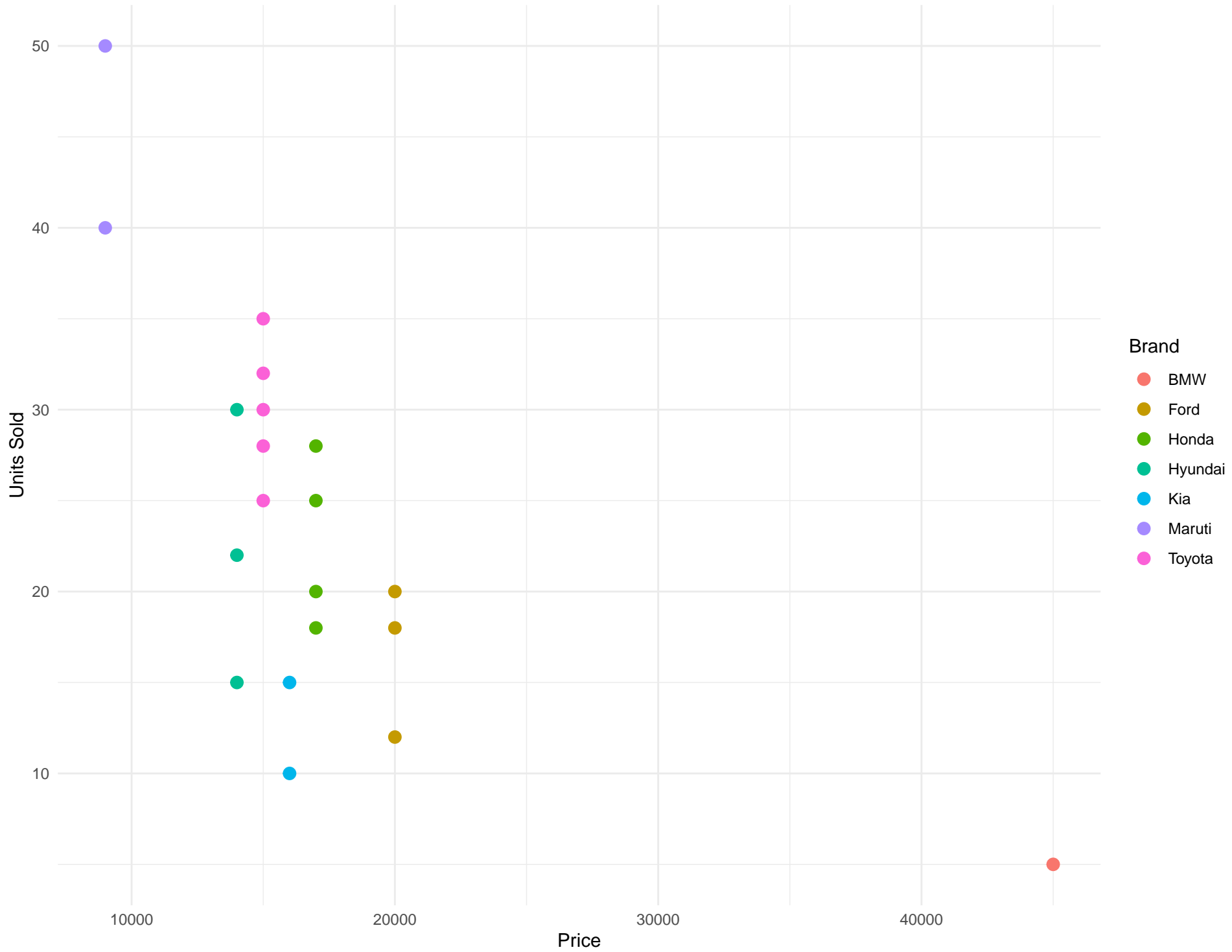
Scatter Plot: Price vs Units Sold
