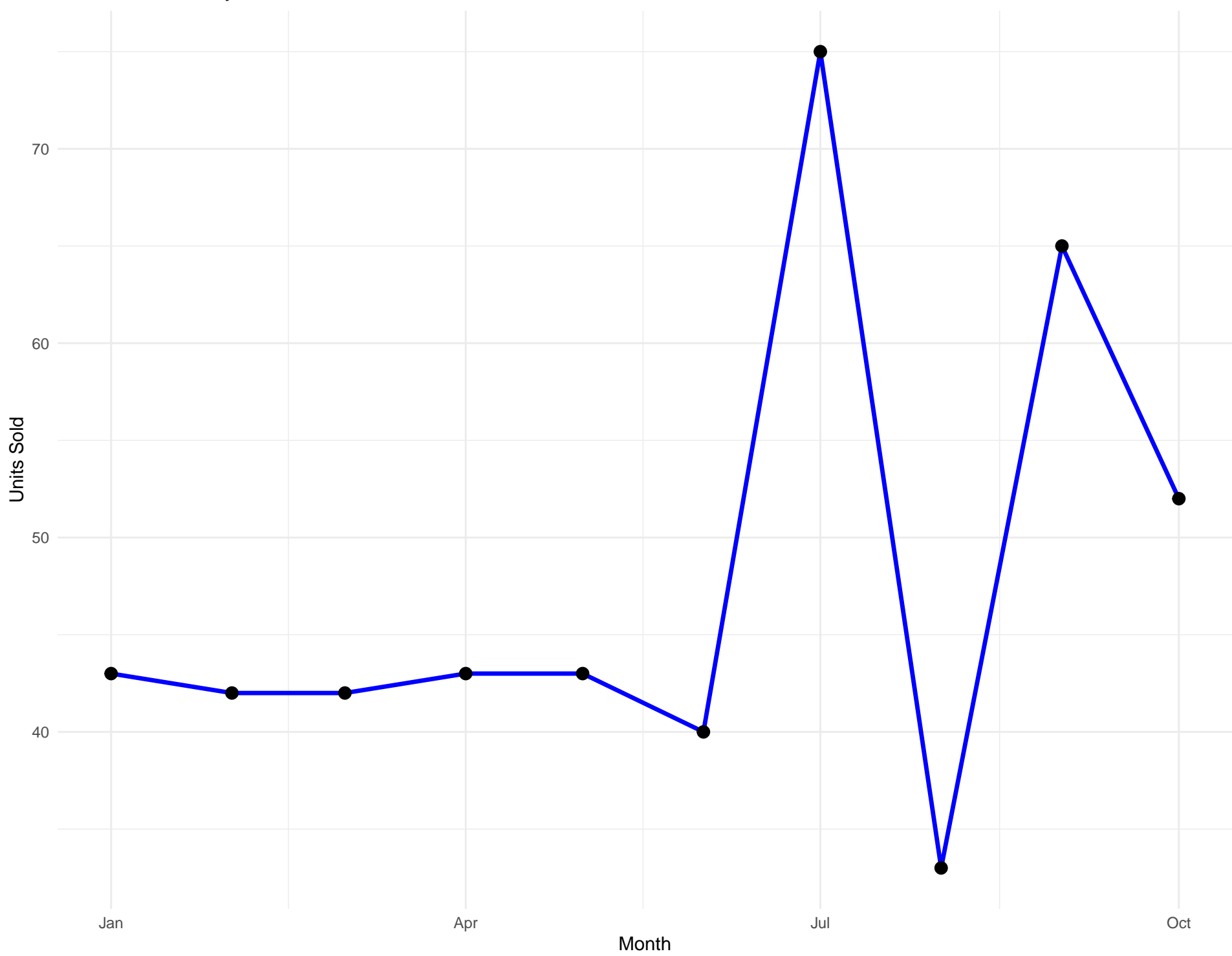
Line Plot: Monthly Sales Trend
