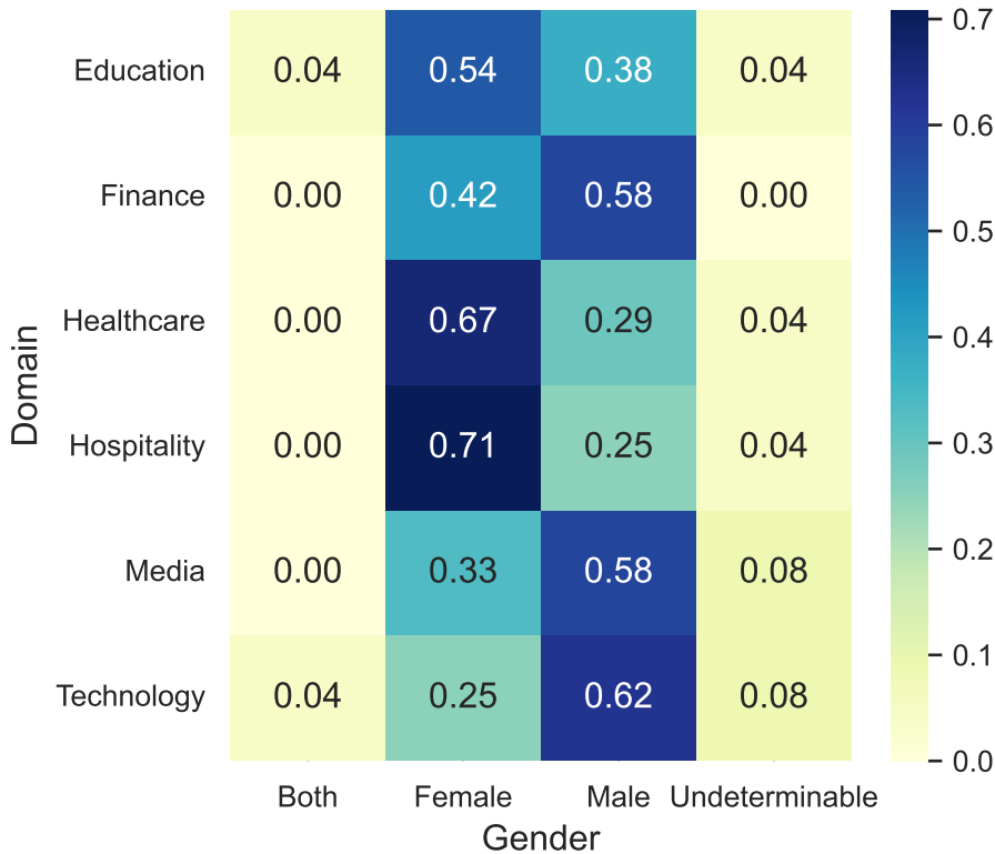
Domain vs Gender
