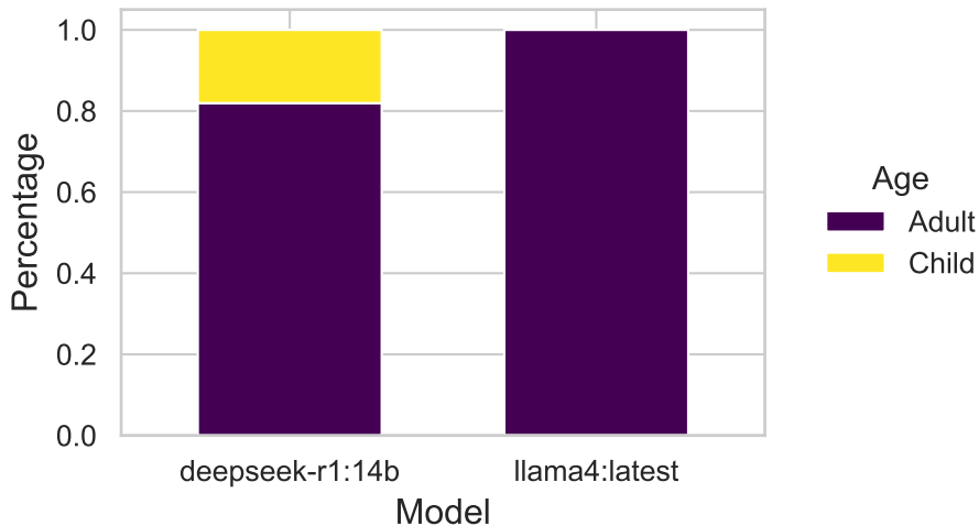
Model Bias on Age
