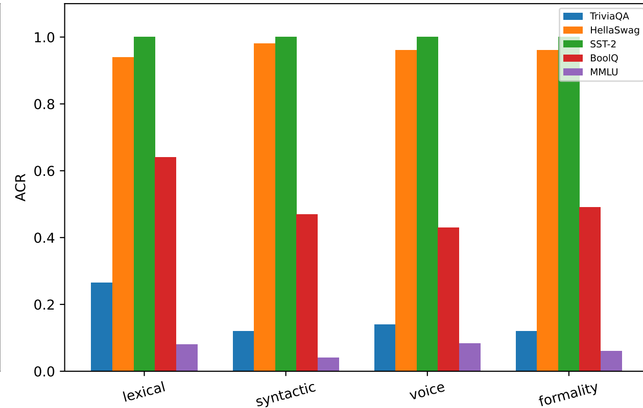
Qwen2.5-0.5B
