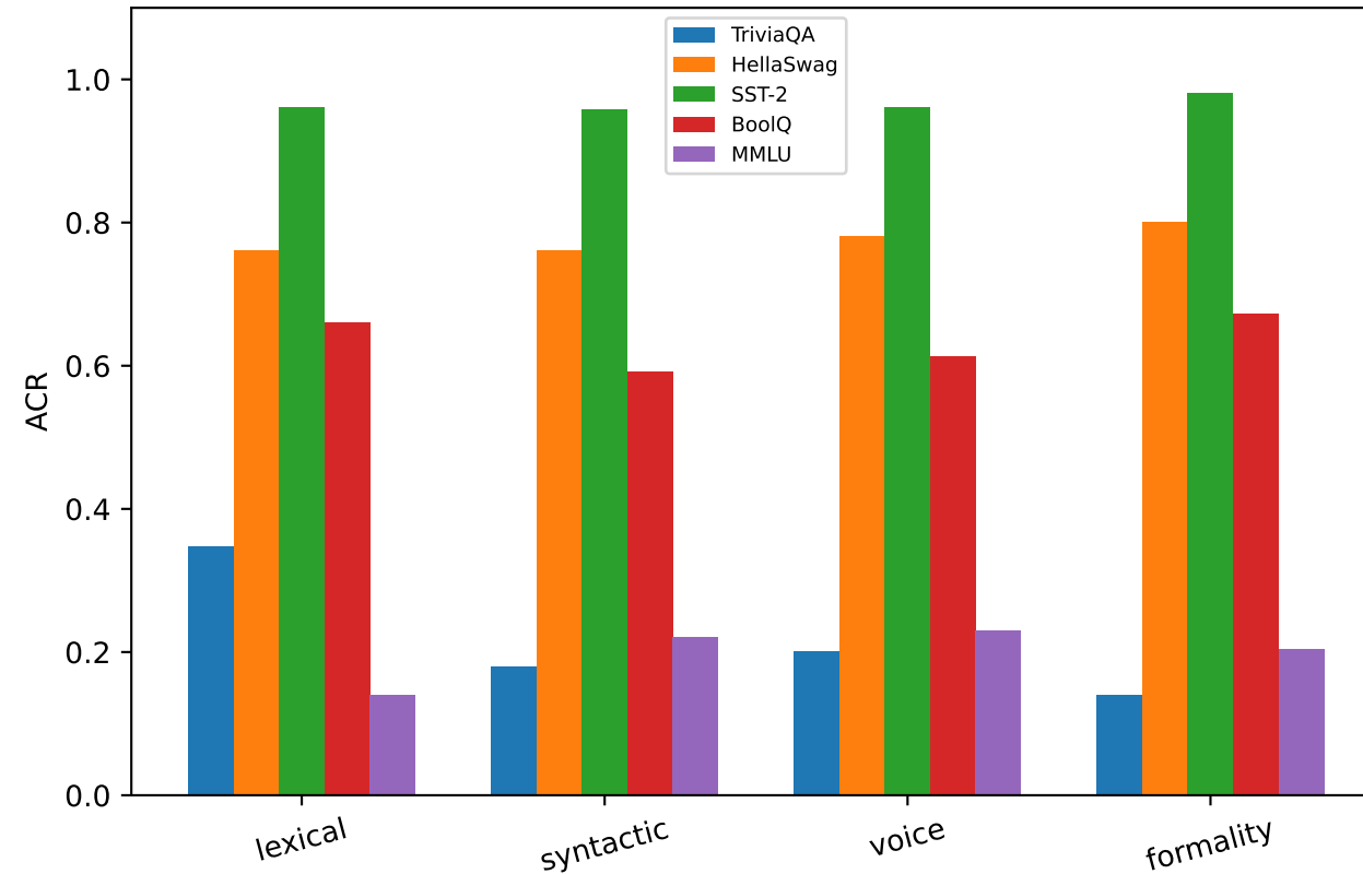
Qwen2.5-1.5B
