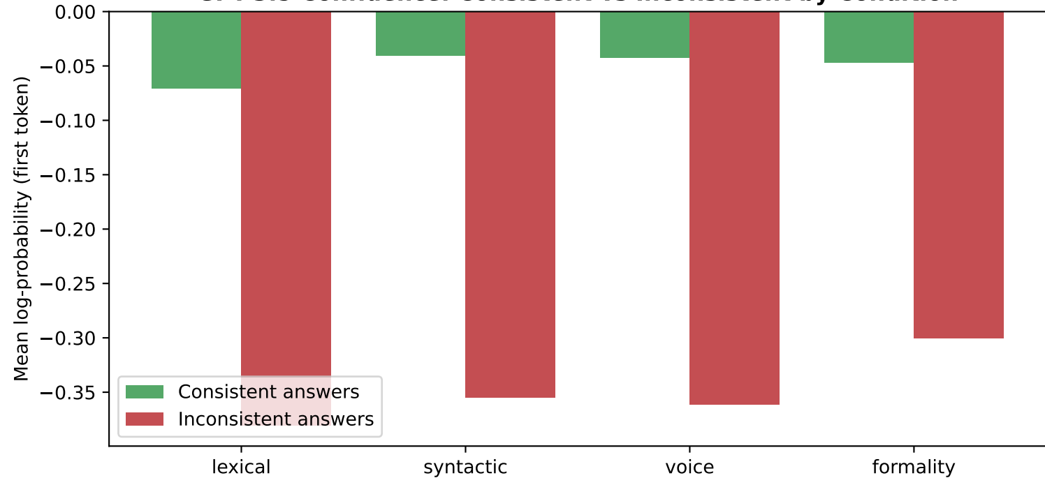
GPT-3.5 Confidence: Consistent vs Inconsistent by Condition
