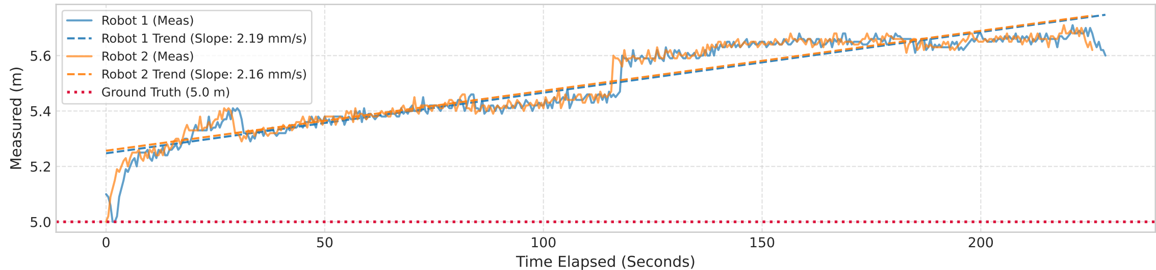
Distance Trajectory & Drift over Time @ True Distance = 5.0 m
