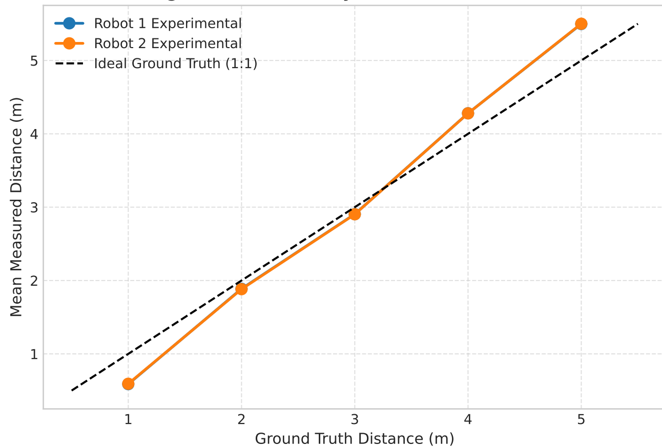
Metrological Scale Linearity: Measured vs True Distance
