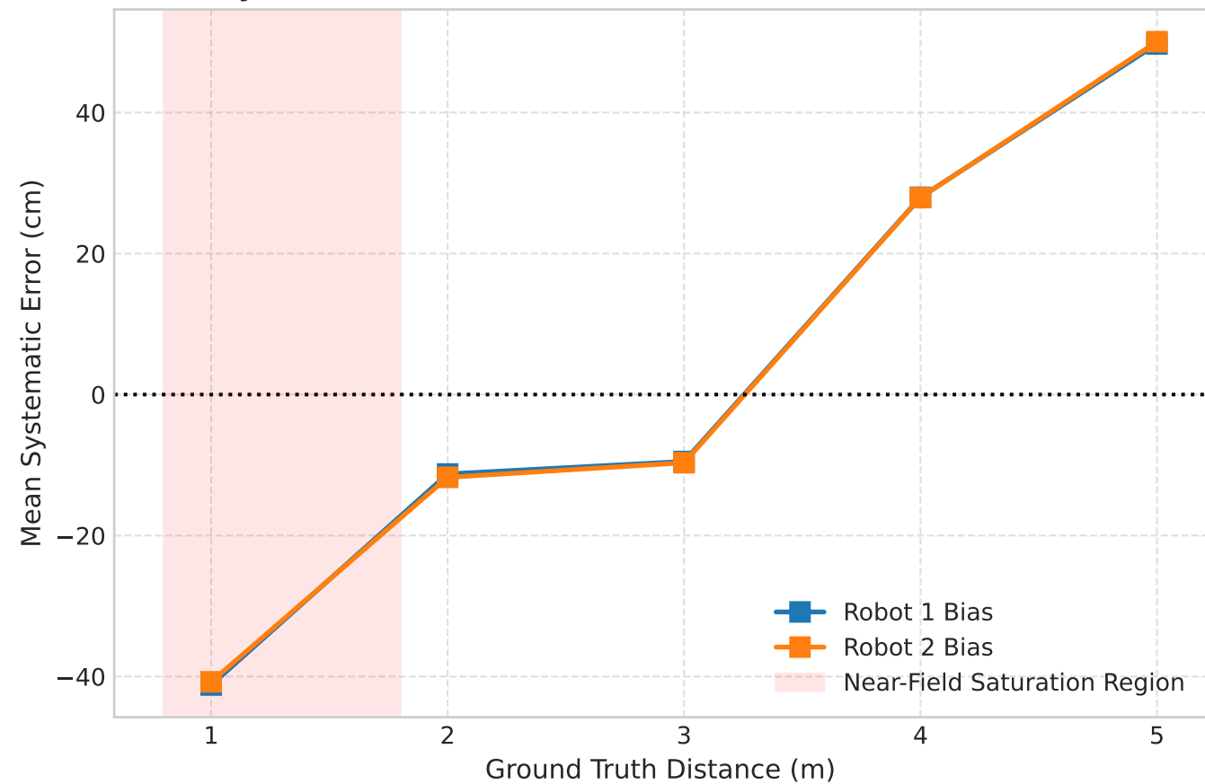
Systematic Measurement Error (Bias) vs True Distance
