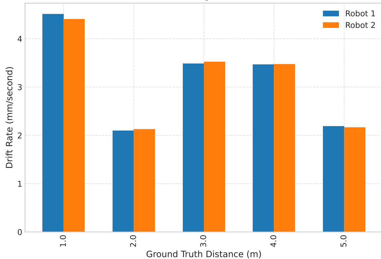
Clock/Thermal Drift Velocity (mm/s) Across Distances
