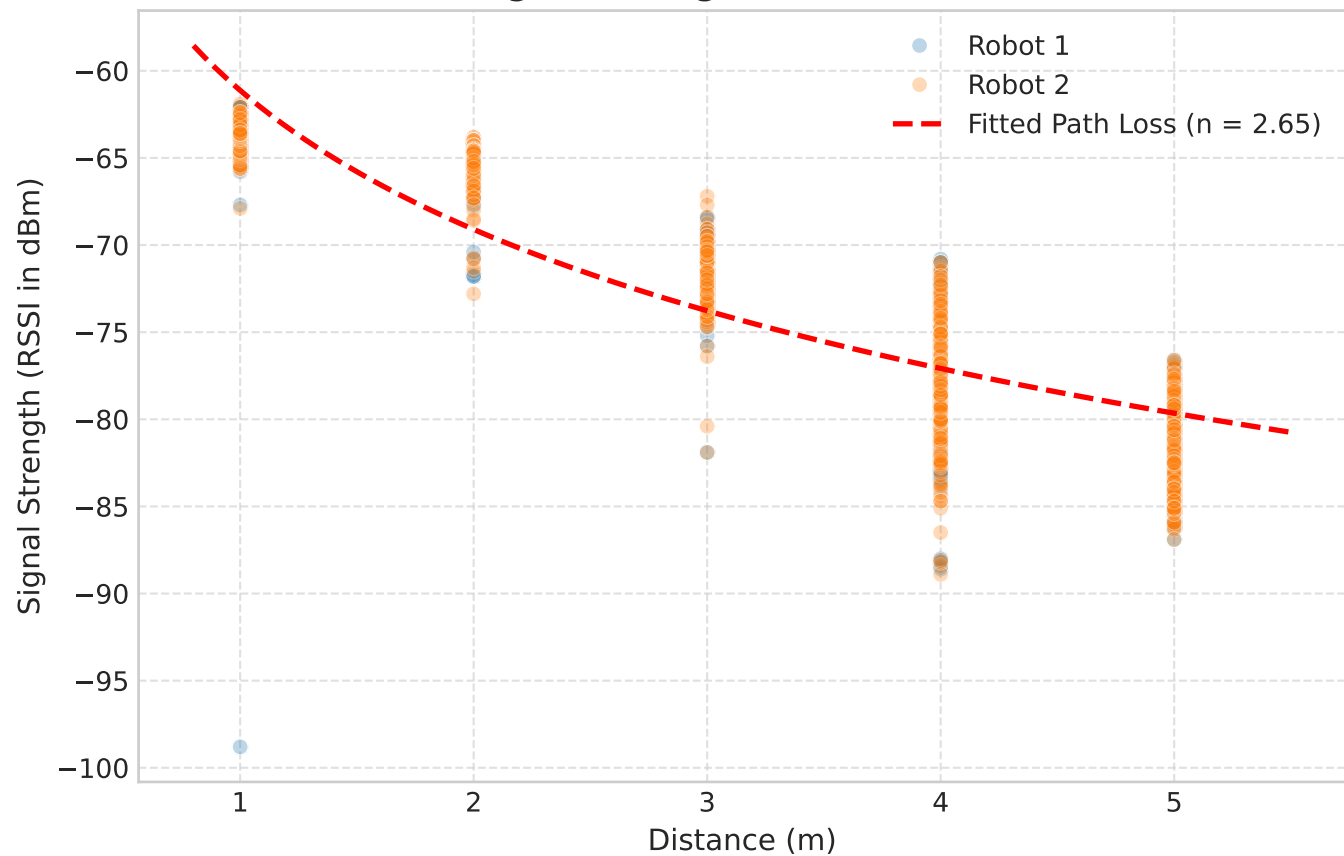
Received Signal Strength (RSSI) vs True Distance
