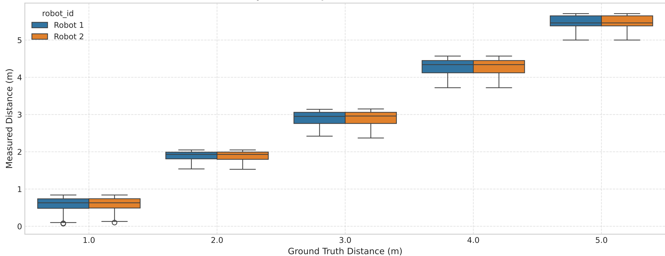
Statistical Dispersion and Jitter Distribution across Distances
