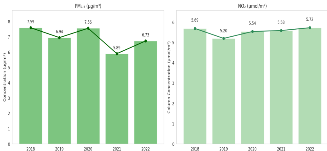
Figure 2.4: Annual PM_{2.5} and NO_2 Trends in Marlborough District
