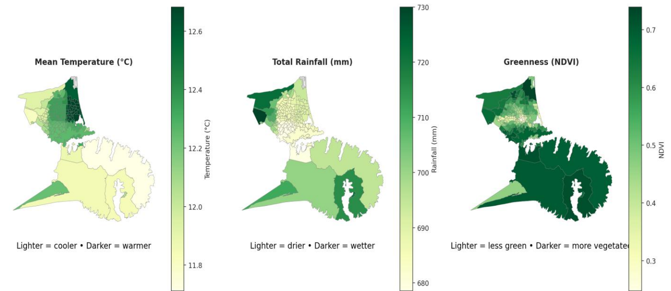
Figure 2.2: Temperature, rainfall, and greenness (NDVI) variation within Christchurch City.
