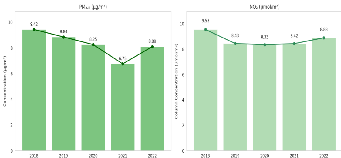
Figure 2.4: Annual PM_{2.5} and NO_2 Trends in Christchurch City
