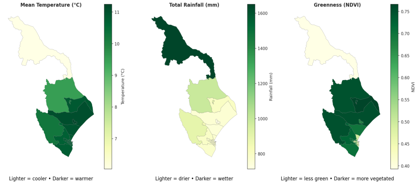
Figure 2.2: Temperature, rainfall, and greenness (NDVI) variation within Timaru District.
