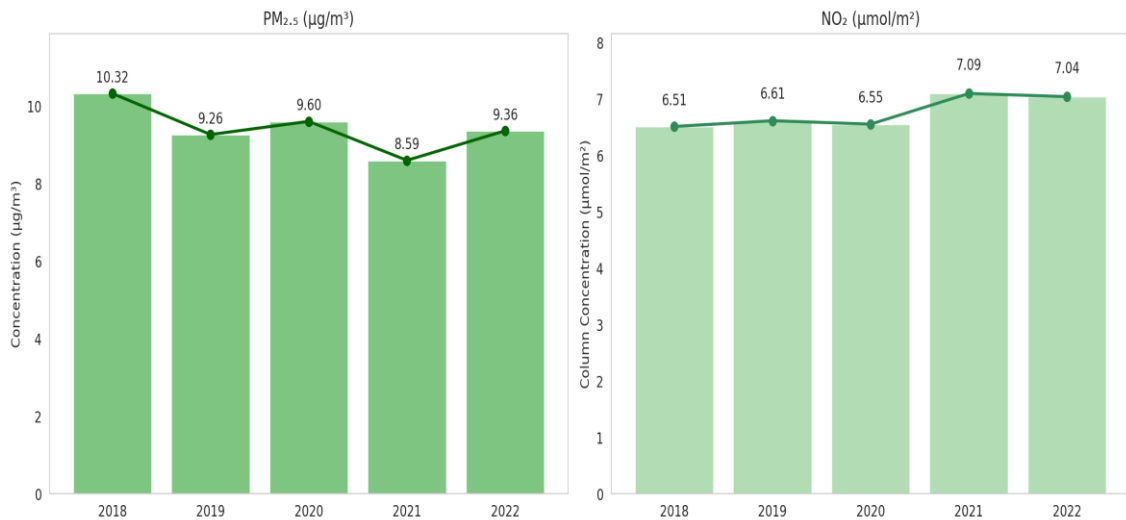
Figure 2.4: Annual PM_{2.5} and NO_2 Trends in Timaru District
