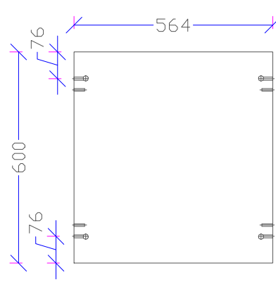
BOTTOM PANEL:564X600X17 FROSTY WHITE-1PCS
