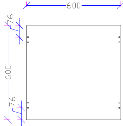
TOP PANEL:600X600X25 CASTLE OAK-1PCS
