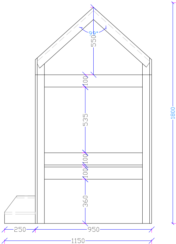
SIDE ELEVATION
