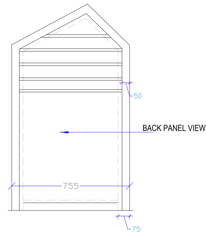
BACK ELEVATION
