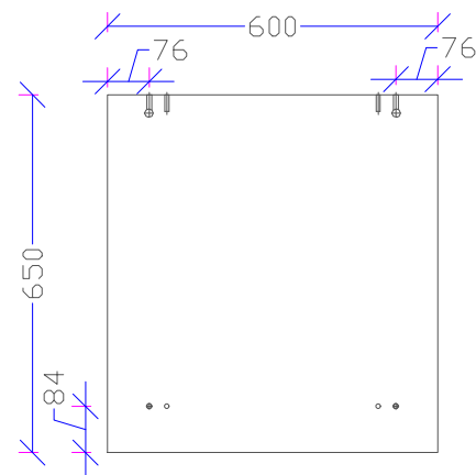
SIDE LEG:600X650X17 CASTLE OAK-2PCS
