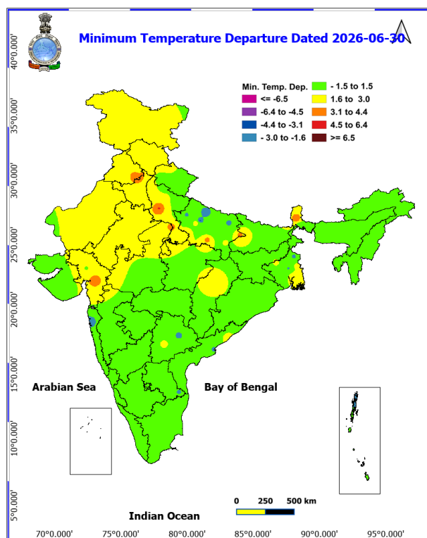
Fig. 4: Departure of Minimum Temp. Dated 2026-06-30
