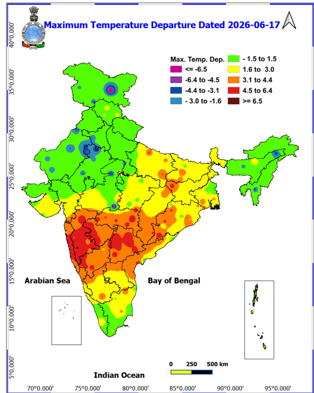
Fig. 2: Departure of Maximum Temp. Dated 2026-06-17
