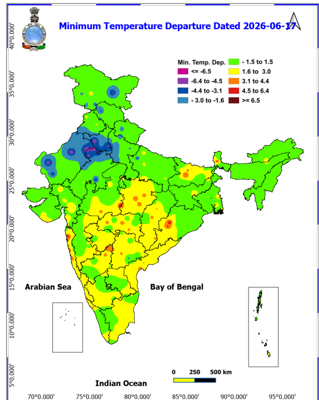
Fig. 4: Departure of Minimum Temp. Dated 2026-06-17
