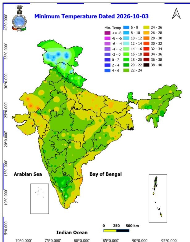
Fig. 3: Minimum Temperatures Dated 2026-10-03
