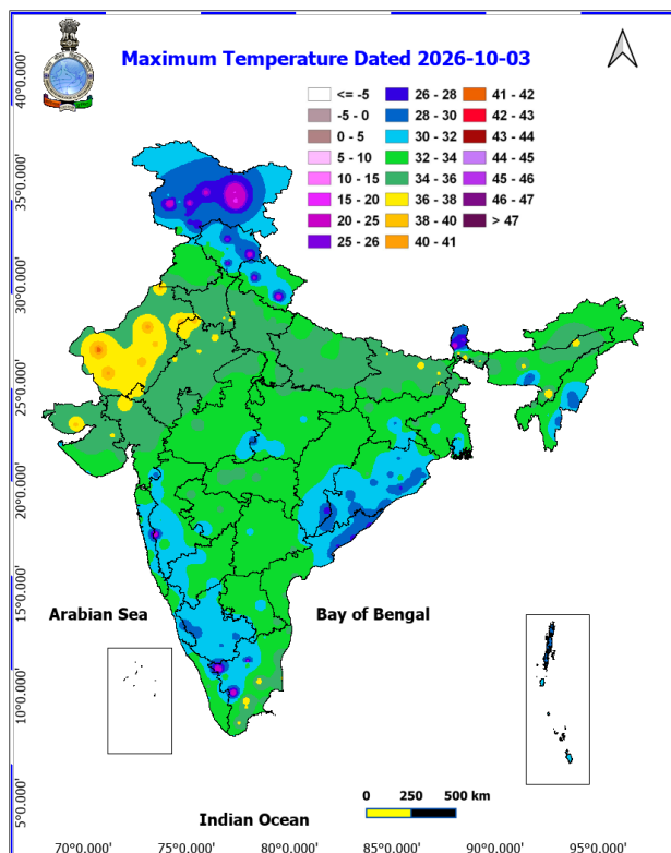
Fig. 1: Maximum Temperatures Dated 2026-10-03
