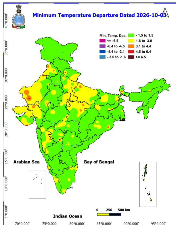
Fig. 4: Departure of Minimum Temp. Dated 2026-10-03
