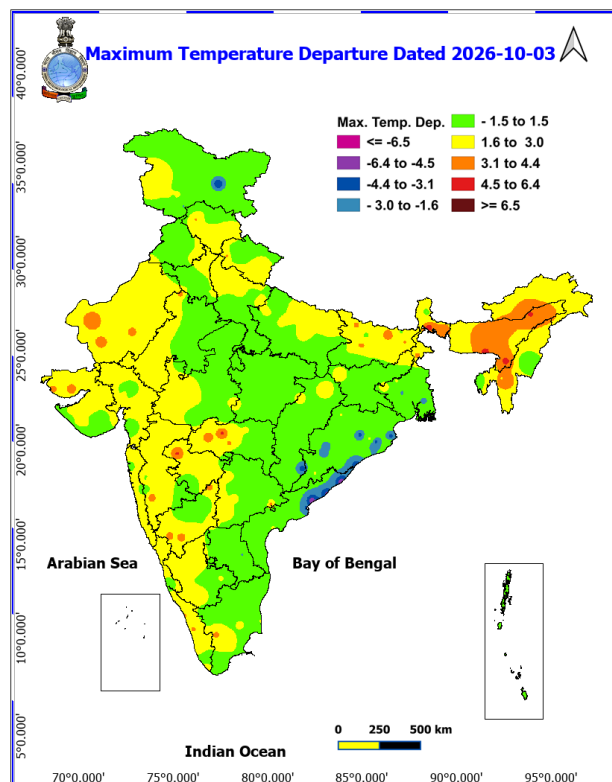
Fig. 2: Departure of Maximum Temp. Dated 2026-10-03
