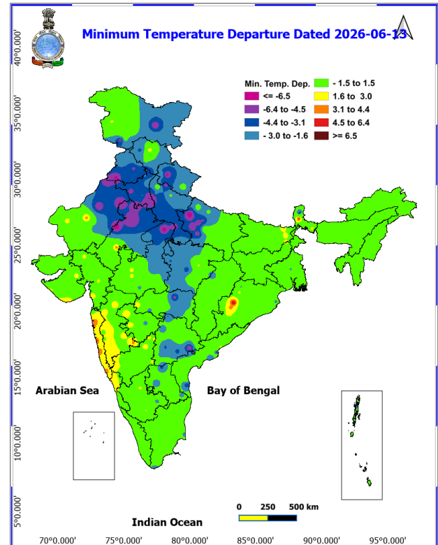
Fig. 4: Departure of Minimum Temp. Dated 2026-06-13
