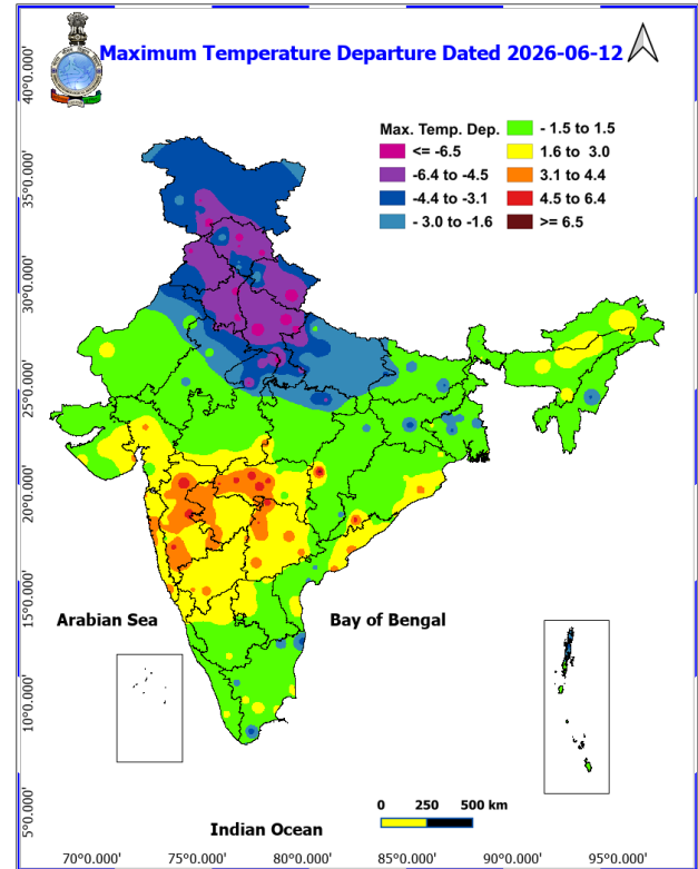
Fig. 2: Departure of Maximum Temp. Dated 2026-06-12
