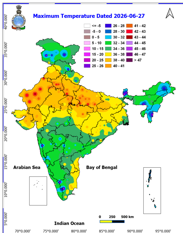
Fig. 1: Maximum Temperatures Dated 2026-06-27
