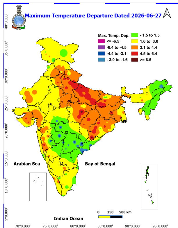
Fig. 2: Departure of Maximum Temp. Dated 2026-06-27
