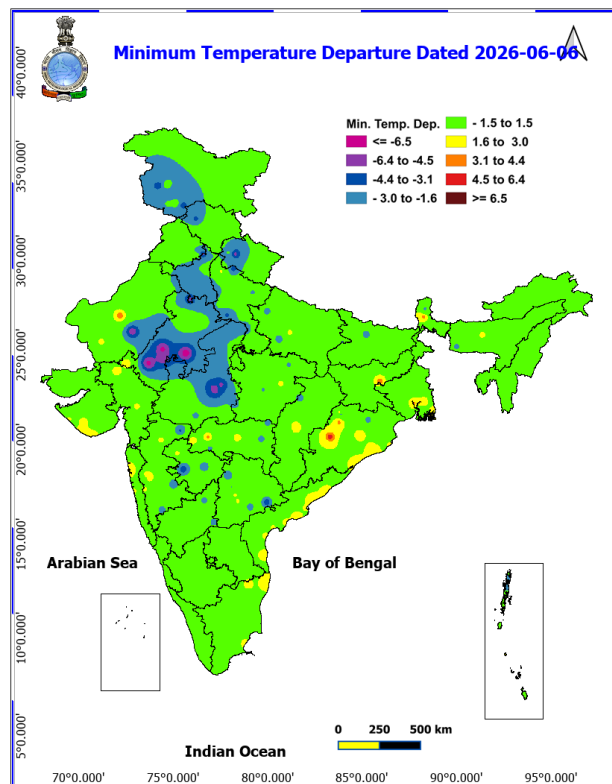
Fig. 4: Departure of Minimum Temp. Dated 2026-06-06
