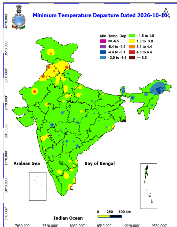
Fig. 4: Departure of Minimum Temp. Dated 2026-10-10
