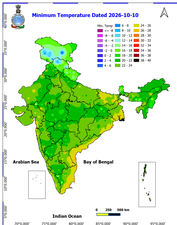
Fig. 3: Minimum Temperatures Dated 2026-10-10
