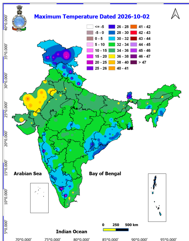
Fig. 1: Maximum Temperatures Dated 2026-10-02
