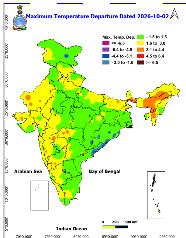
Fig. 2: Departure of Maximum Temp. Dated 2026-10-02
