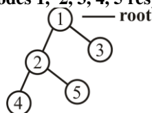
Tree - T
