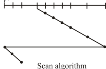
Scan algorithm
